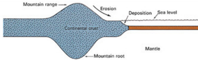
Figure 3: Another illustration shows how the mountains are peg-like in shape, due to their deep roots. 1923
