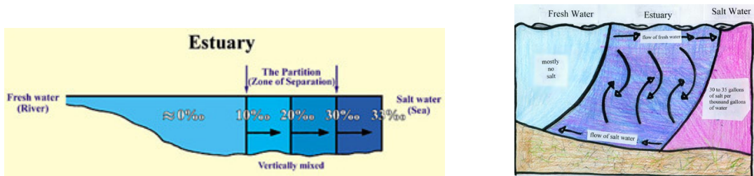
Figure 2: Longitudinal section showing salinity (parts per thousand ‰) in an estuary. We can see here the partition (zone of separation) between the fresh and the salt water. 1913
