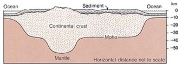
Figure 1: Mountains have deep roots under the surface of the ground. 1921
