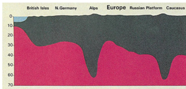
Figure 2: Schematic section. The mountains, like pegs, have deep roots embedded in the ground. 1922
