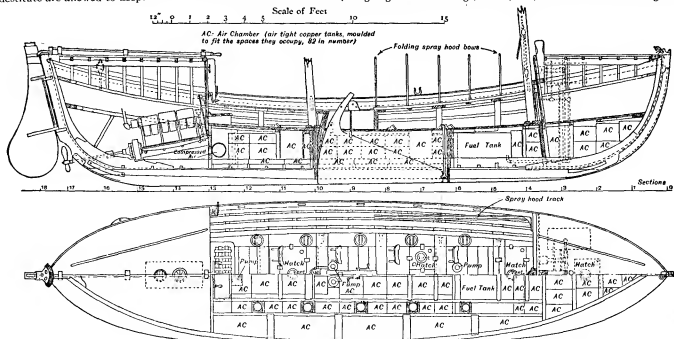
FIG. 10.—American Power Life-boat.
