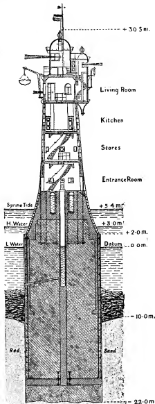
FIG. 21.—Rothersand Lighthouse.
