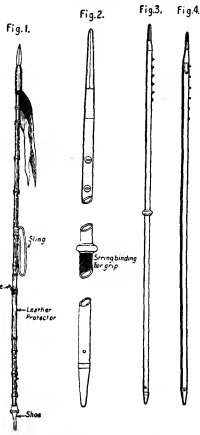
Fig. 1 is the British bamboo lance; figs. 2 and 3 the German steel tubular lance, and fig. 4 the German pine-wood lance.
