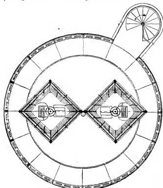
FIG. 43A.—Le Vierge Apparatus and Lantern. Plan at focal plane.
