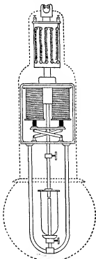
FIG. 8.—Enclosed Arc Lamp.
