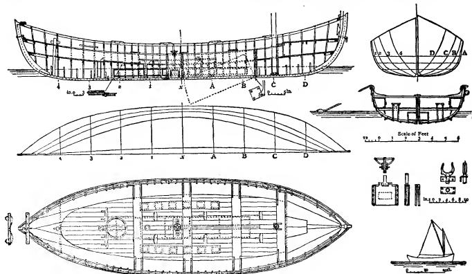
FIG. 11.—Beebe-McLellan Self-bailing Boat.
