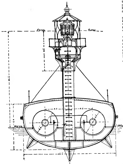
FIG. 49.—Otter Rock Light-vessel.
