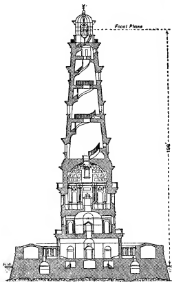
FIG. 1.—Cordouan Lighthouse.
