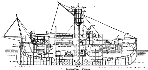
FIG. 47.—Sandettié Lightship.
