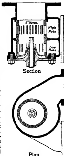
Fig. 53.—St Catherine's Double-noted Siren.
