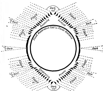
FIG. 45.—Isle of May Apparatus.
