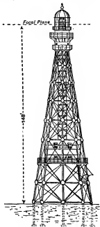
FIG. 26.—Cape San Thomé Lighthouse.
