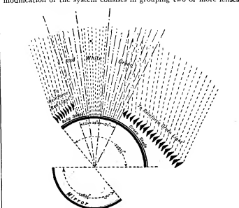
FIG. 38.—Gage Roads Direction Light.
