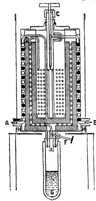
FIG. 2.—Laboratory Liquid Air Machine.
