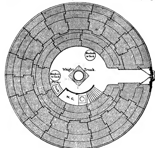
FIG. 6.—Plan of Entrance Floor, Eddystone Lighthouse.
