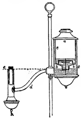
FIG. 2.—Section of Reading Lamp.
