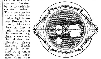
FIG. 39.—Pendeen Apparatus. Plan at Focal Plane.
