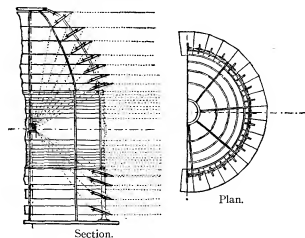
FIG. 35.—Fixed Apparatus at Chassiron Lighthouse (1827).
