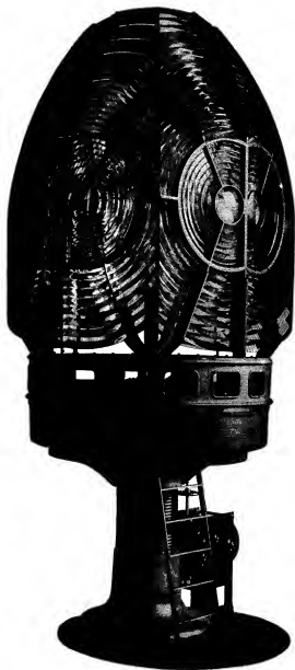
FIG. 55.—PACHENA POINT LIGHTHOUSE, B.C.—FIRST ORDER DOUBLE-FLASHING APPARATUS.
