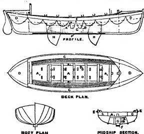
FIG. 8.—Plans, Profile and Section of Watson Deck and Life-boat. Lettering as in fig. 5, but C, side air-cases above deck and thwarts.
