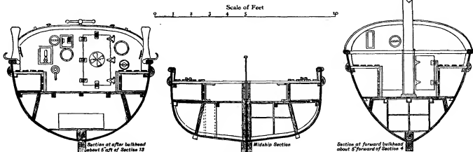
FIG. 12.—Details of boat shown in Fig. 10.
