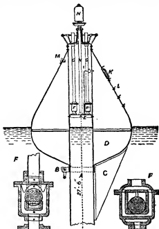
FIG. 51.—Courtenay's Automatic Whistling Buoy.
