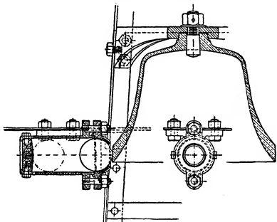
FIG. 52.—Buoy Bell.
