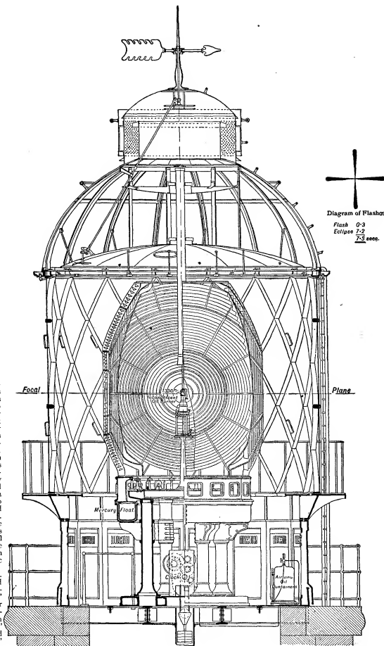
FIG. 41.—Manora Point Apparatus and Lantern.
