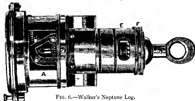
FIG. 6.—Walker's Neptune Log.
