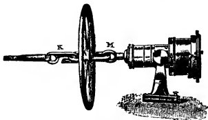
FIG. 11.—Neptune Log fitted with Governor.
