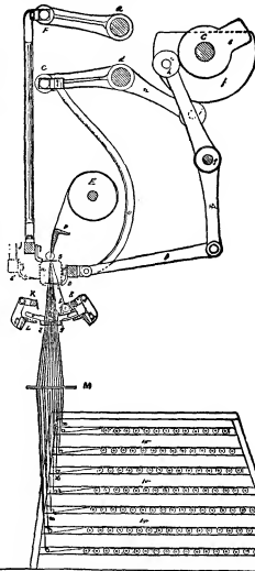
FIG. 49.—Section of Lace Machine.
