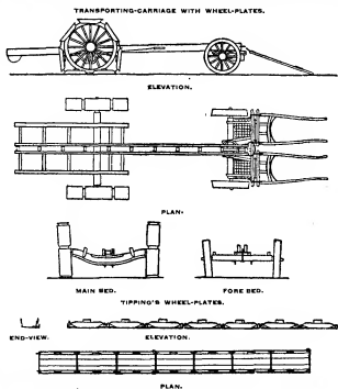
FIG. 9.—Life-boat Transporting-Carriage with Tipping's Wheel-Plates.
