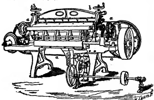
FIG. 7.—Band Knife Splitting Machine.
