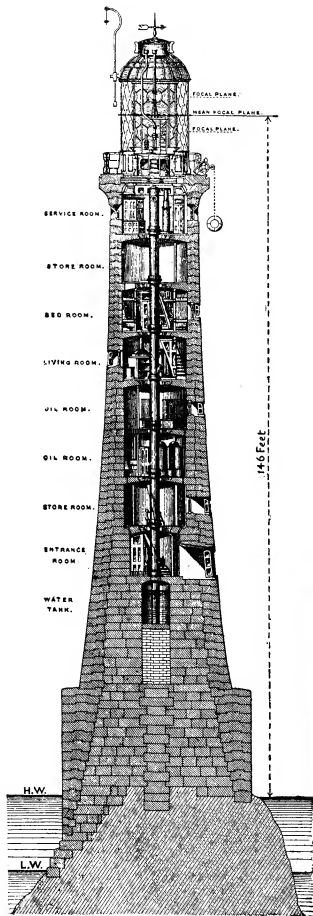
FIG. 13.—Bishop Rock Lighthouse.
